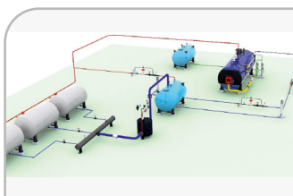
HIGH PRESSURE CONDENSATE RECOVERY SYSTEM
